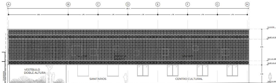
Fachada Principal
