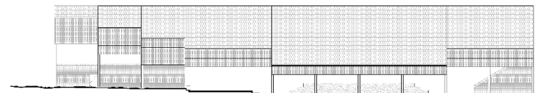
Fachada principal
