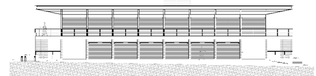
Fachada General
